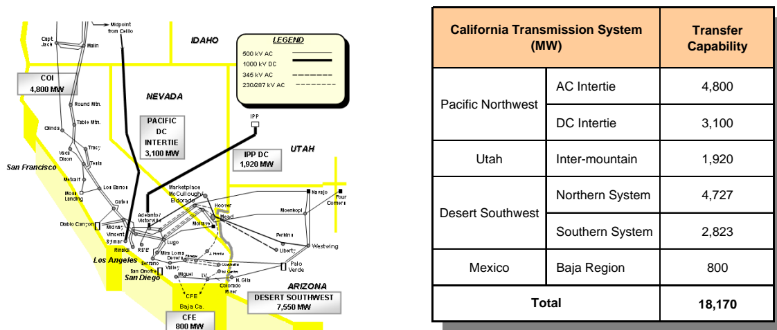
Figure 11 California's 18,170 MW (18.2 GW) of EHV Transmission Interconnections
